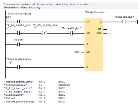
(i) Example 2-wire or FBD for Sorting Station Scenario
