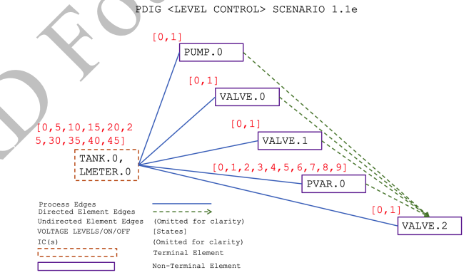
(a) Example PDIG Model for the Level Control Process of the FL Attack Incident
