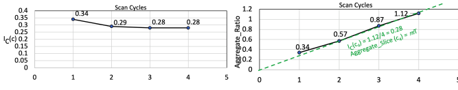
(c) A plot of I_C(s) to scan cycles (d) Plot of Aggregate Slices to scan cycles
