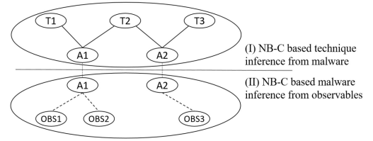
Fig. 5. Framework of multi-layer naïve Bayesian inference of initial hypotheses within AttackDB.
