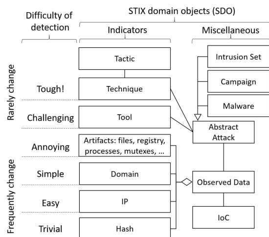
Fig. 1. AttackDB schema with detection difficulties according to the Pyramid of Pain.
