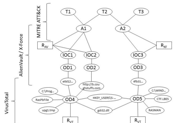
Fig. 3. An illustration of AttackDB's structure.
