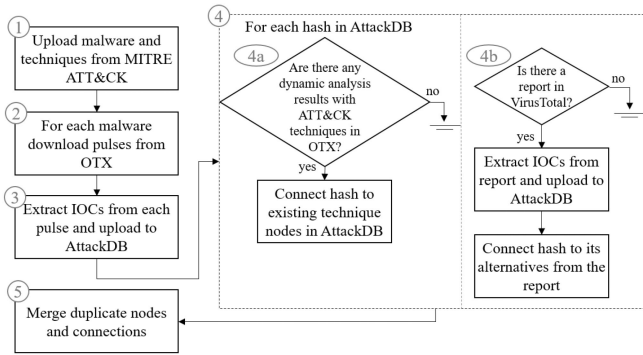
Fig. 2. Flow chart of AttackDB's construction.
