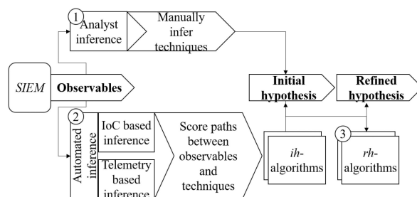
Fig. 4. Overview of the hypothesis generation process.
