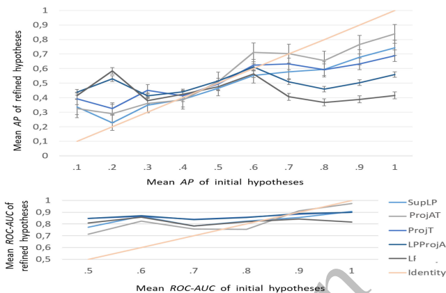
Fig. 10. Mean AP and ROC - AUC of refined hypotheses depending on the precision of the initial hypotheses.
