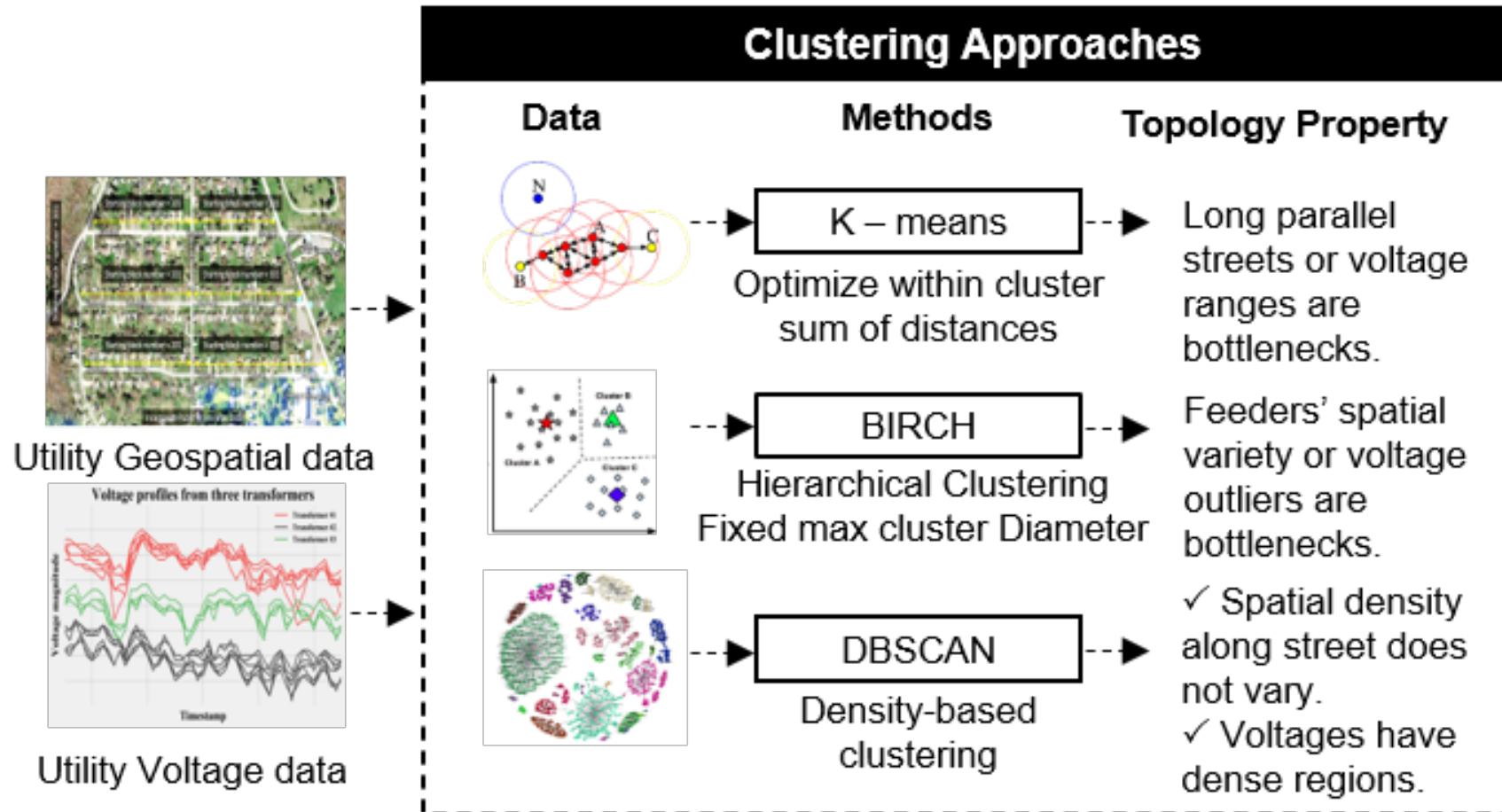
Fig. :Comparison of three important families of algorithms for clustering based on both GIS and AMI data.
